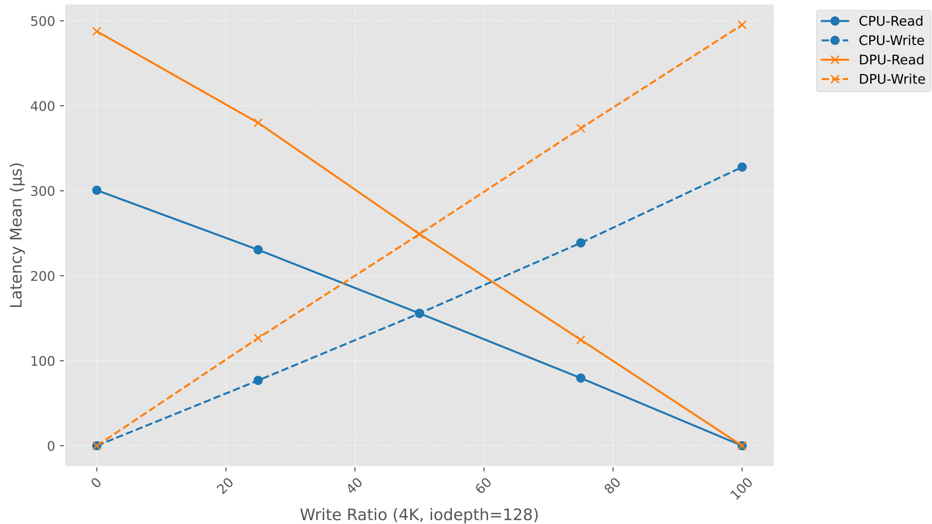
Latency Mean vs Write Ratio (4K, iodepth=128)
